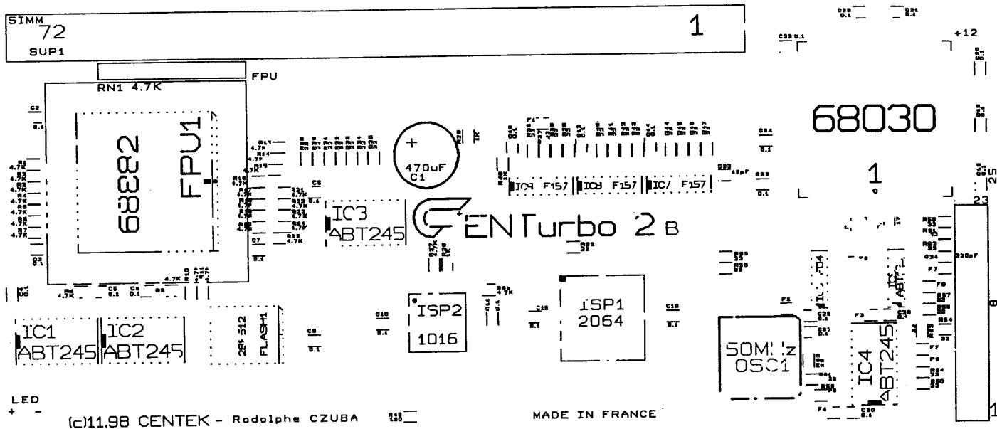
Top Vernish mask
